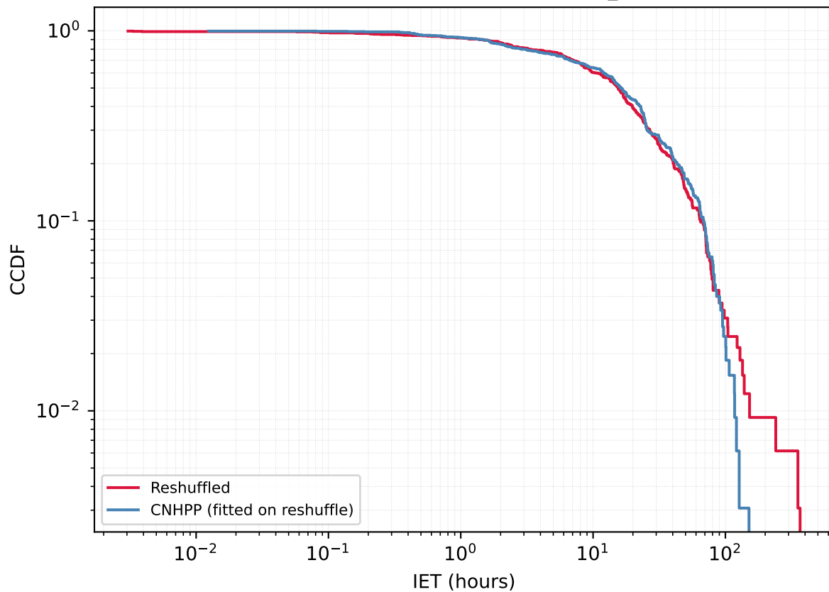
User 302926911 - Reshuffled vs CNHPP A_{\text{fit}}=0.2037
